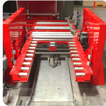
Pallet Lift
