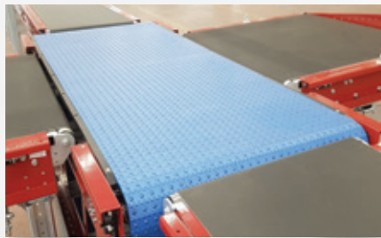
Roll-on sorter (up to 4.000 pcs/hour)
