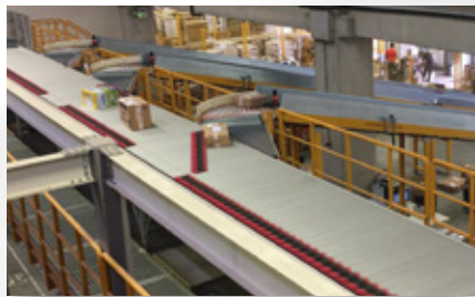
Shoe Sorter (up to 10.000 pcs/hour)
